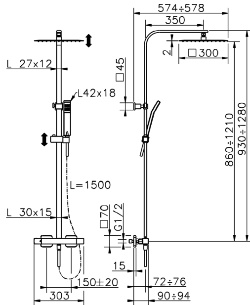
QT C8603H CombiDoccia Termostatico Thermo CombiShower CombiDouche Thermo
