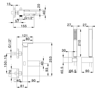
NE 000124 Completo Monocomando Vasca Bath/S. Mixer Set Ensemble Mitigeur Bain/D.
