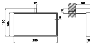
SQ 090220 Porta Salviette Towel Rail Porte-Serviette
