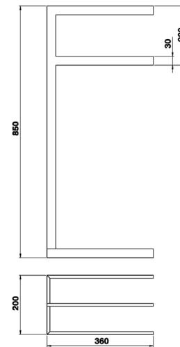
SQ 090910 Porta Salviette Free-Standing Towel Rail Porte-Serviette
