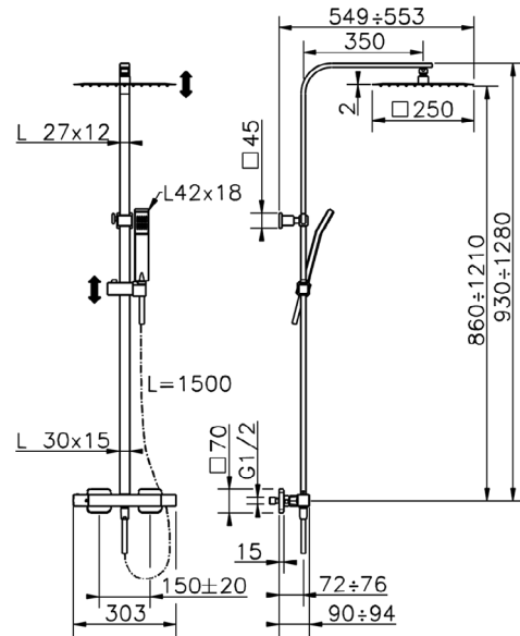
QT C8602H CombiDoccia Termostatico Thermo CombiShower CombiDouche Thermo
