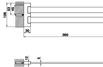
SQ 090210 Porta Salviette Towel Rail Porte-Serviette
