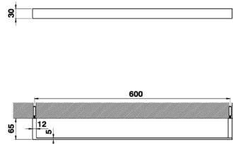
SQ 090106 Porta Salviette Towel Rail Porte-Serviette
