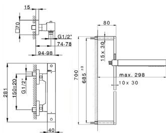
NE S01010 Completo Termostatico Doccia Thermo Shower Set Ensemble Thermo Douche
