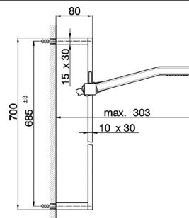
SS 010040 Completo Doccia Saliscendi Slide Rail Shower Set Ensemble Barre de Douche
