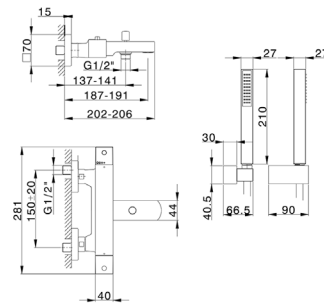
NE D27010 Completo Termostatico Vasca Thermo Bath/S. Set Ensemble Thermo Bain/D.
