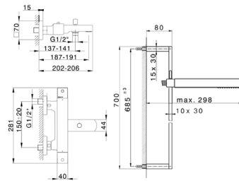
NE S27010 Completo Termostatico Vasca Thermo Bath/S. Set Ensemble Thermo Bain/D.
