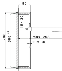
SS 010860 Completo Doccia Saliscendi Slide Rail Shower Set Ensemble Barre de Douche
